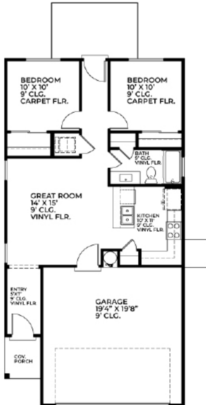
MAIN FLOOR PLAN MAIN FLOOR - 800 SQ. FT. GARAGE AREA - 400 SQ. FT. COV. PORCH - 30 SQ. FT.
