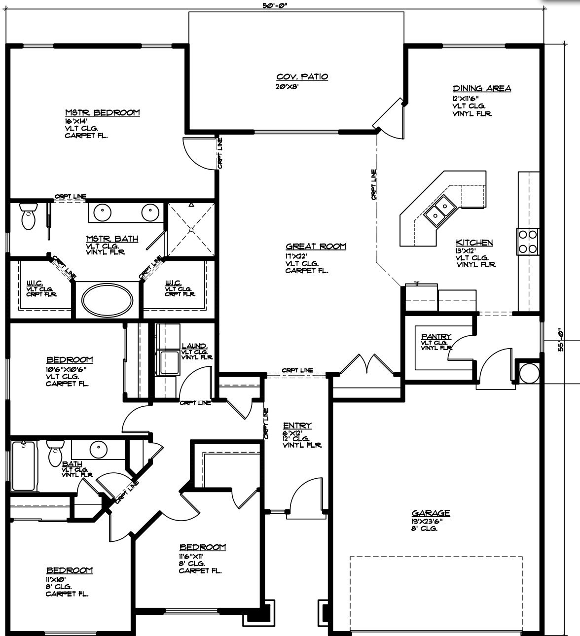
MAIN FLOOR PLAN MAIN FLOOR 2044 SQ. FT. GARAGE AREA 436 SQ. FT.
